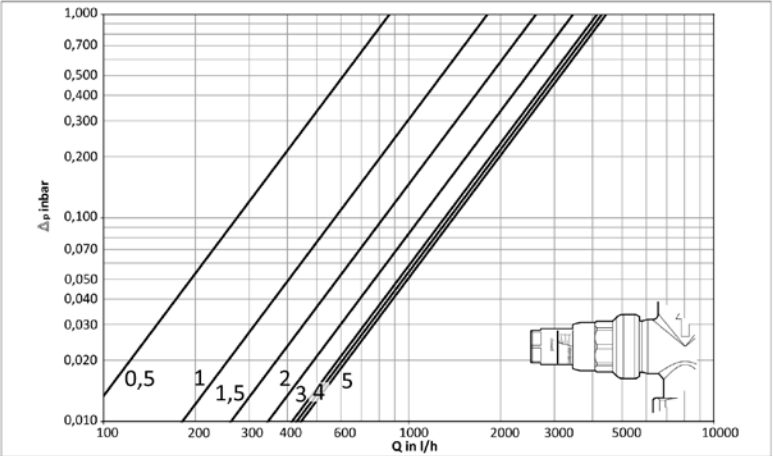
Figure 4: Balancing valve
